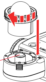
Lumisphere Lock Lever ⑳
