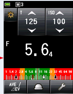
Measuring Screen
