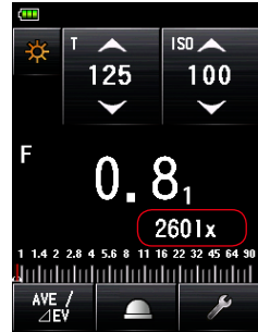
Measuring Screen Additional data for illuminance / luminance
